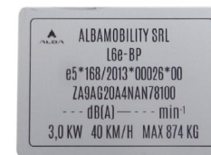
EMBLEMS AND LABELS EMBLEMI ED ETICHETTE
