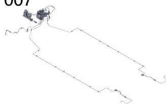
BRAKE SYSTEM IMPIANTO FRENI
